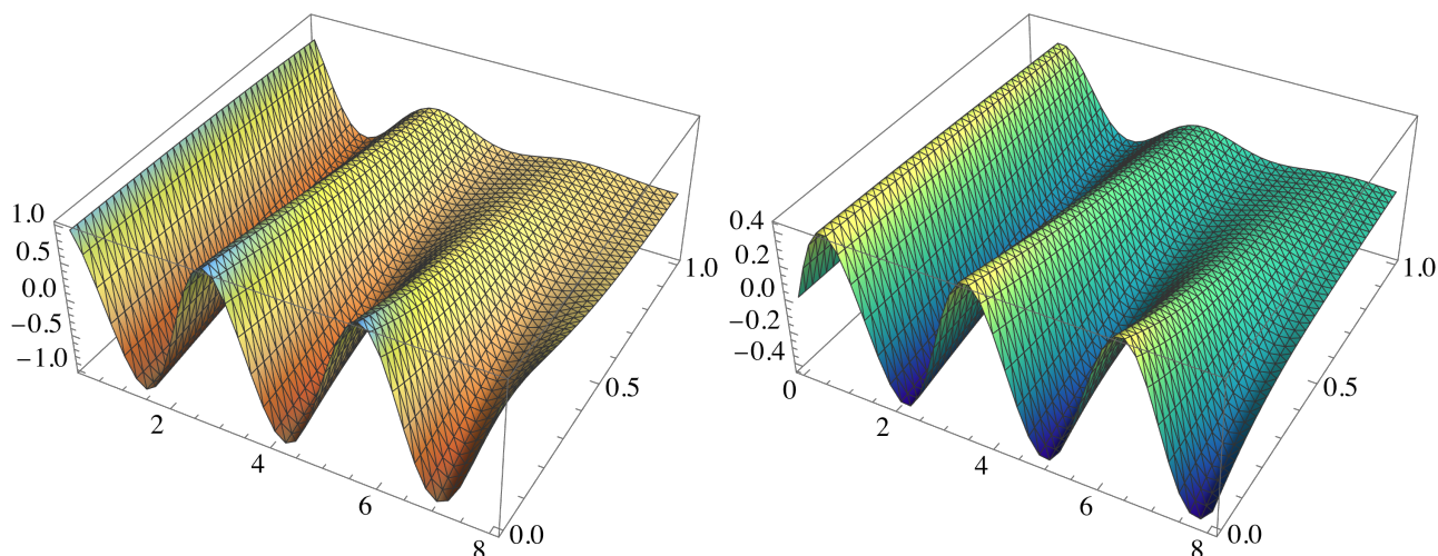
Figure 5. Graphics of the approximations x_{\text{likecos}}^{(N)}(t, \alpha) (left) and x_{\text{likesin}}^{(N)}(t, \alpha) (right) for 0 < t < 8 , 0 < \alpha < 1 , when \omega_\alpha = 1 , \omega_0 = 2 , and N = 40 .
