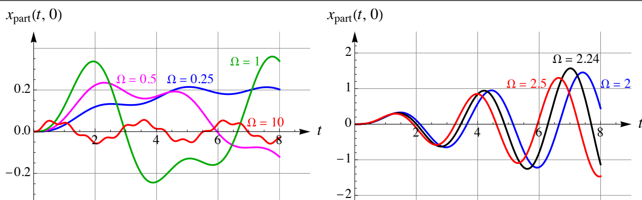
Figure 9. Graphics of x_{\text{part}}(t, 0) for \Omega = 0.25, 0.5, 1, 10 (left) and \Omega = 2, 2.4, 2.5 (right) for 0 < t < 8 , when \omega_\alpha = 1 and \omega_0 = 2 .
