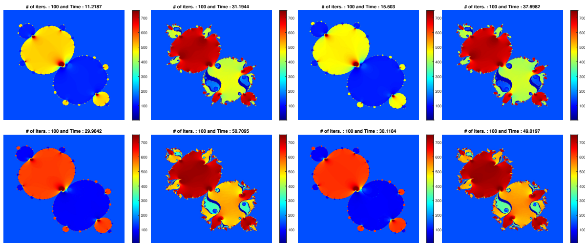
Figure 12: Example 4.7 for \alpha_n = \alpha_n^1 = \alpha_n^2 = \alpha_n^3 = 0.9 for all n \in \mathbb{N}_0 , \theta = 0.5 , accuracy \epsilon ps = 1 , the area being [-20, 20]^2 , the iteration count fixed at 100 and \omega = 0.009i : (from left to right): Algorithms CJP, JPI (ver. 2), CJM, JMI (ver. 2) (first line); Algorithms CJI, JII (ver. 2), CJNS, JNSI (ver. 2) (second line)
