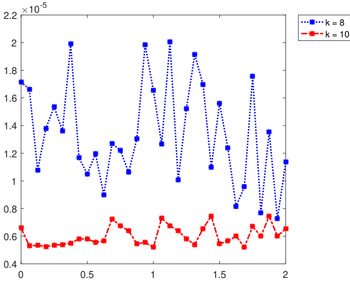
FIGURE 10. Errors at the non-negative nodes for k = 8 and k = 10 iterations
