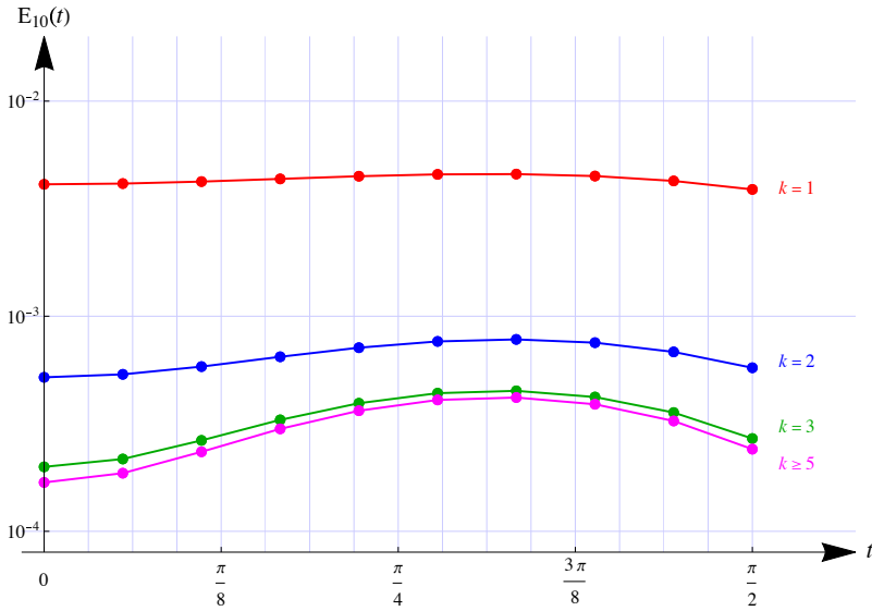
FIGURE 4. Errors at n+2=10 equidistant nodes for the trapezoidal rule and k=1, 2, 3 and k \geq 5 iterations
