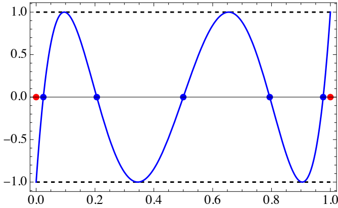
FIGURE 2. Zeros of T_n(2t - 1) for n = 5 as internal nodes and additional zeros at 0 and 1
