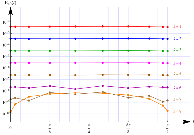
FIGURE 8. Errors at the Clenshaw-Curtis n + 2 = 10 nodes for the rules and k = 1, 2, \dots, 8 iterations
