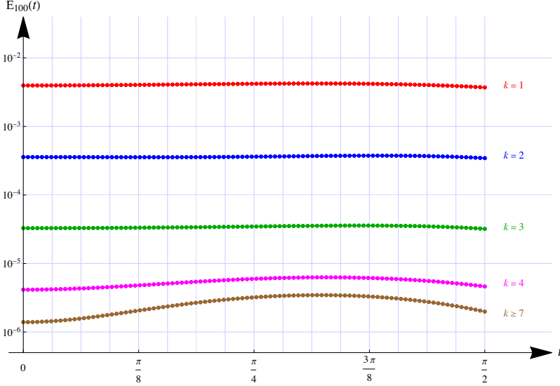
FIGURE 6. Errors at n + 2 = 100 equidistant nodes for the trapezoidal rule and k = 1, 2, 3, 4 and k \geq 7 iterations
