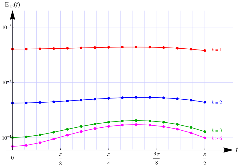
FIGURE 5. Errors at n+2=15 equidistant nodes for the trapezoidal rule and k=1, 2, 3 and k \geq 6 iterations
