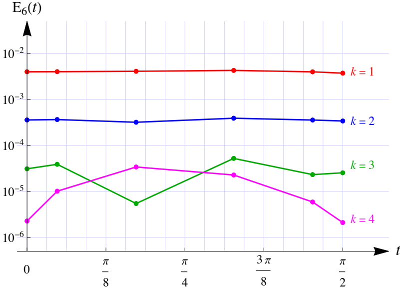
FIGURE 7. Errors at the Clenshaw-Curtis n + 2 = 6 nodes for the rules and k = 1, 2, \dots, 4 iterations
