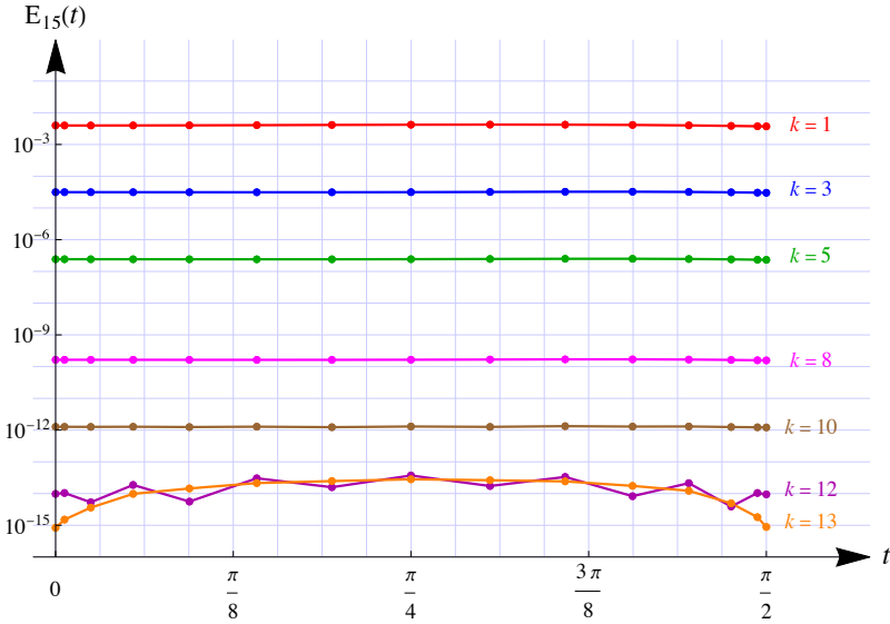
FIGURE 9. Errors at the Clenshaw-Curtis n + 2 = 15 nodes for the rules and k = 1, 3, 5, 8, 10, 12, 13 iterations
