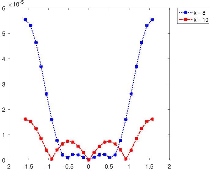
FIGURE 11. Errors at the nodes for k = 8 and k = 10 iterations
