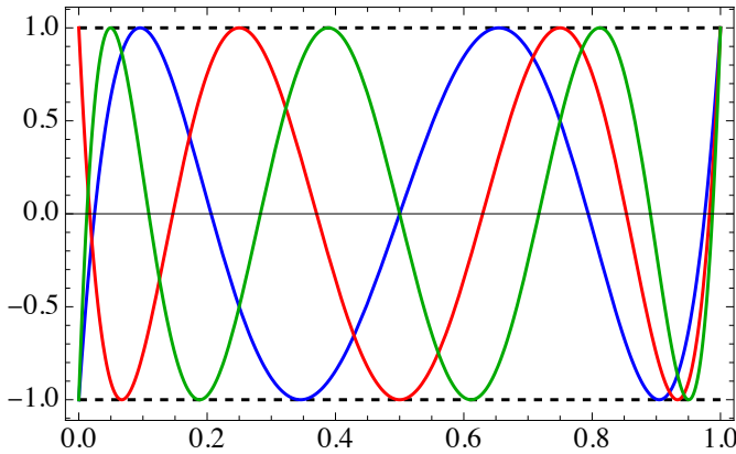
FIGURE 1. Chebyshev polynomials T_n(2t - 1) transformed to [0, 1] for n = 5 (blue), n = 6 (red), and n = 7 (green)
