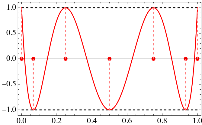
FIGURE 3. Extremal points of T_{n+1}(2t - 1) for n = 5
