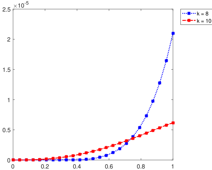
FIGURE 12. Errors at the nodes for k = 8 and k = 10 iterations
