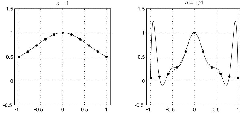
Fig. 2 The Runge's example for n = 11 equally spaced nodes, for a = 1 (left) and a = 1/4 (right)
