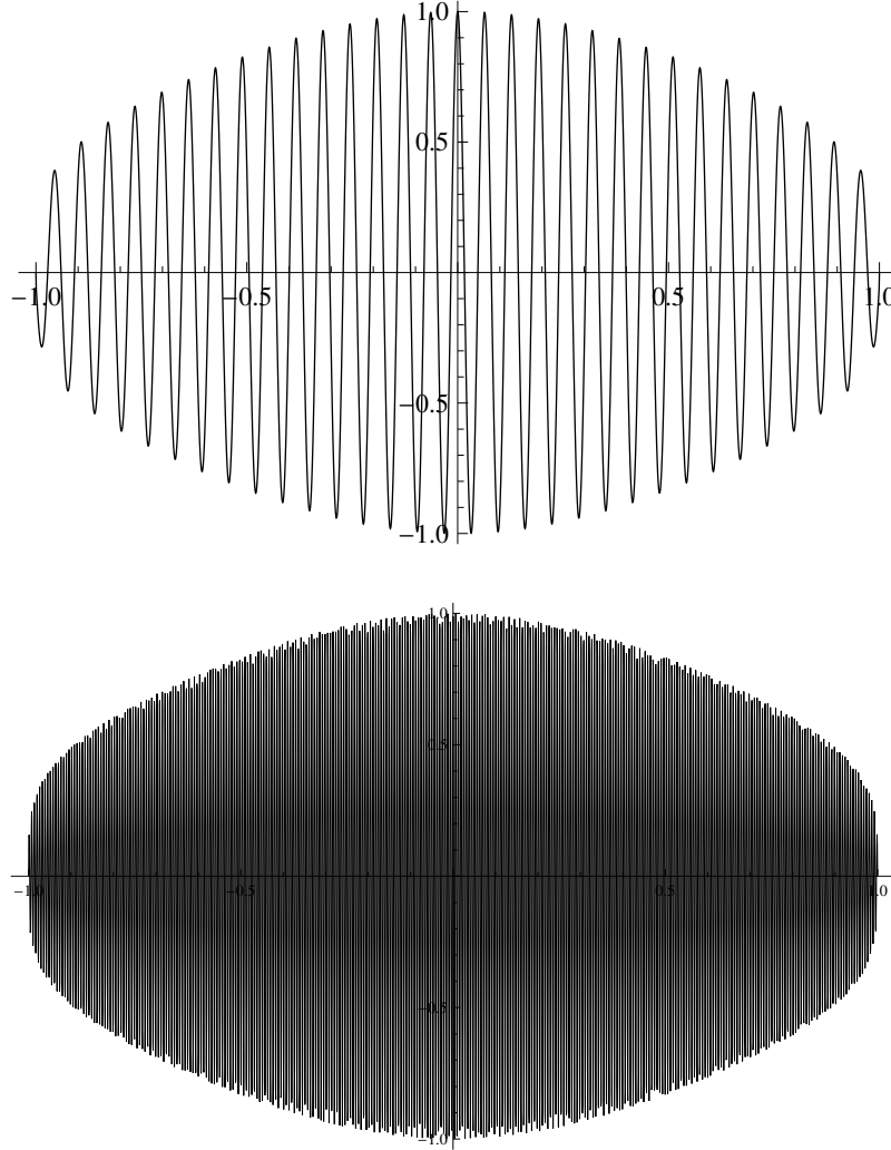
Fig. 1 The graphs of the function \text{Im}((1-x^2)^{1/4}e^{i\zeta x}/(x-i)) for \zeta = \zeta_1 (top) and \zeta = \zeta_2 (down)
