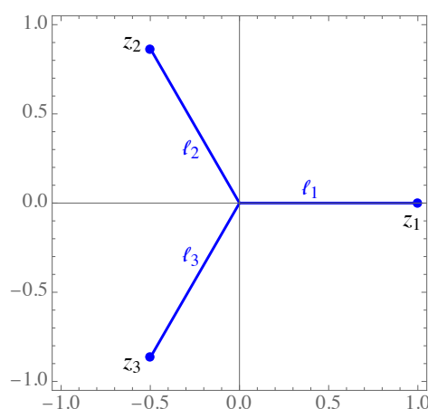
Figure 2. Three rays \ell_1, \ell_2 and \ell_3 in the complex plane, given by the complex points z_s = e^{2i(s-1)\pi/3} , s = 1, 2, 3 .
