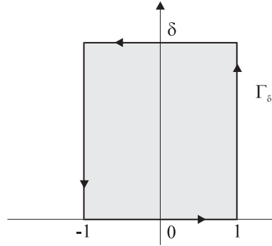
Figure 3.1: The contour of integration
